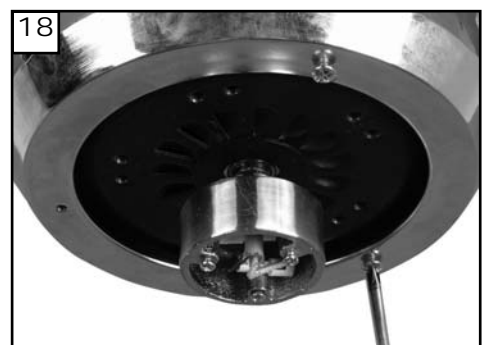
18 Loosen 2 screws with key slots and remove the 1 screw without key slot. Save screw removed.
